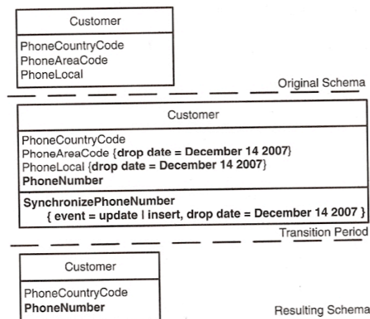
Figure 6.6 Merging columns in the Customer table.
